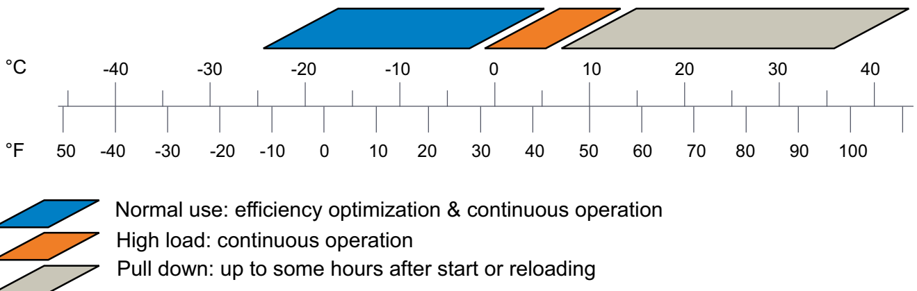
Secop MBP compressors: evaporation pressures
