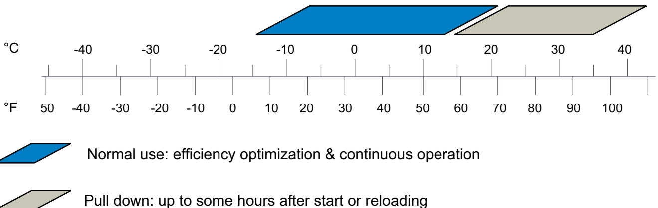
Secop HBP compressors: evaporation pressures
