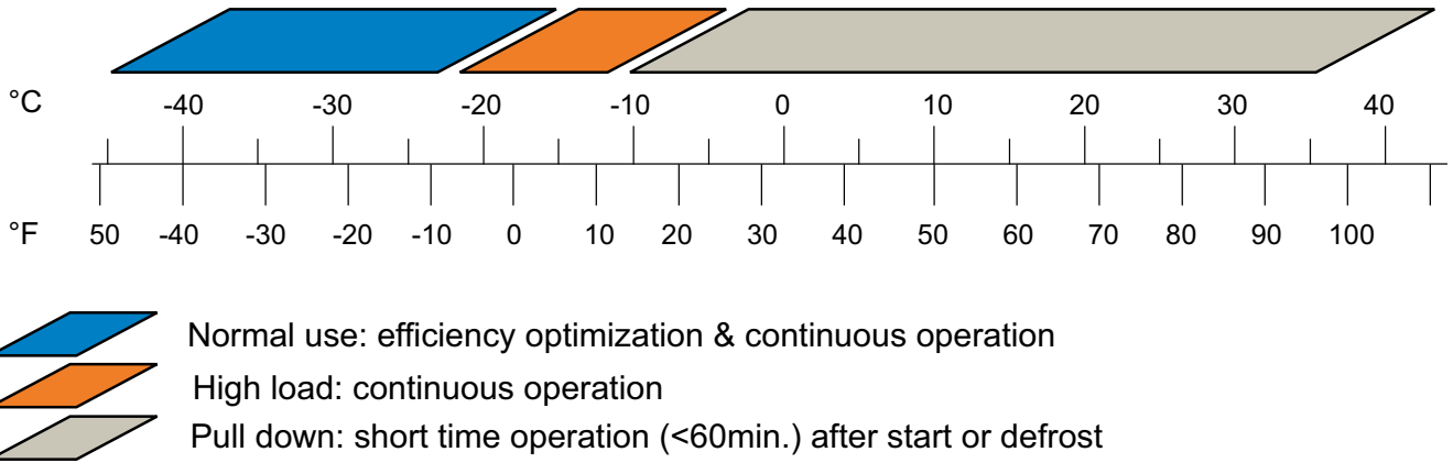
Secop LBP compressors: evaporation pressures
